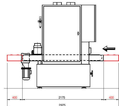
Machine with Longitudinal units with 2 working units
