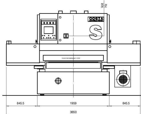
Machine with Cross belt unit and Longitudinal units
