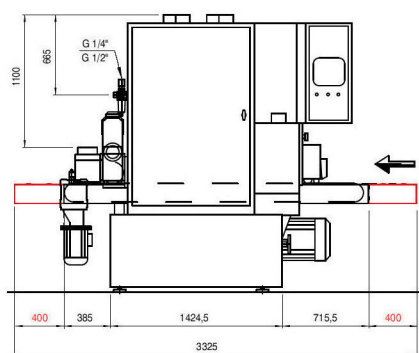
version with 1 cross belt unit and 2 longitudinal units
