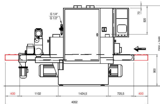
Machine with Longitudinal units with 2 working units
